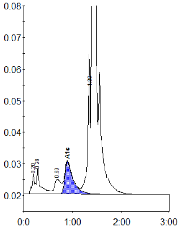
Peak table - ID: 10541760
